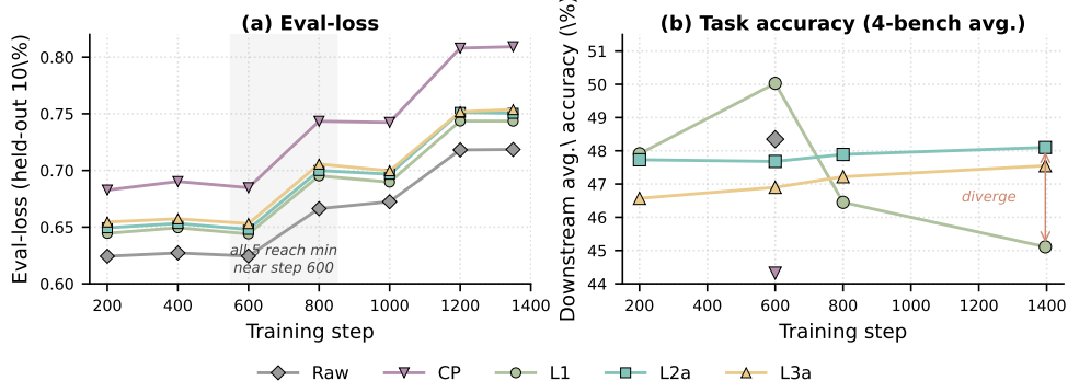
Figure 6: Eval-loss curves (left, dense schedule) vs. downstream 4-benchmark accuracy (right, four evaluated checkpoints) for L1 , L2a , L3a .
