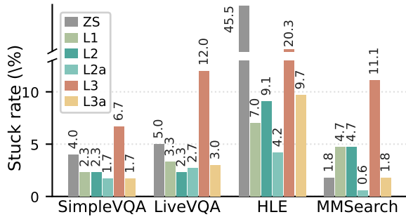
Figure 3: Stuck rate (%), the fraction of samples that hit the 128-round agent-loop ceiling.
