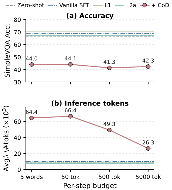
Figure 4: Chain-of-Draft sweep on SimpleVQA versus Zero-shot, Vanilla SFT, L1 , and L2a .
