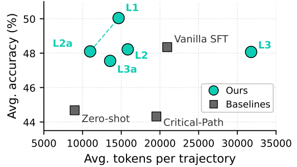
Figure 1: Accuracy vs. inference-cost trade-off. L1 reaches the highest accuracy. L2a halves the inference tokens at vanilla-SFT accuracy.
