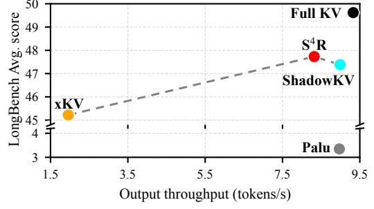
Figure 1: Performance–speed trade-off on Qwen3-4B. The y-axis is broken to include the dominated Palu.
