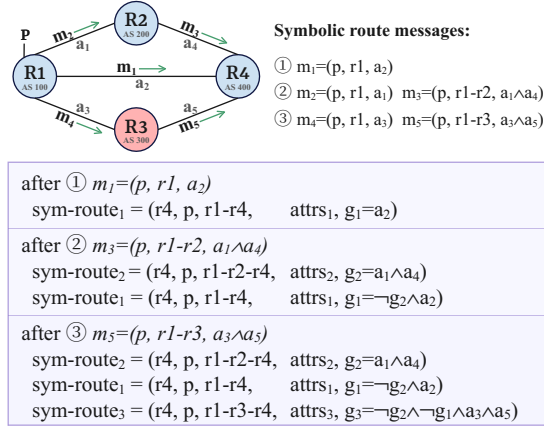
Figure 4: Symbolic route generation.
