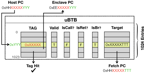
Figure 7: Host and enclave branches map to same uBTB entry.
