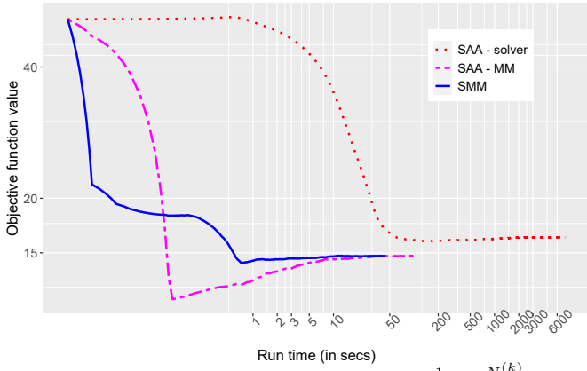
Fig. 1. Convergence comparisons for objective value \frac{1}{N^{(k)}} \sum_{i=1}^{N^{(k)}} \ell(\theta, \xi_i) .
