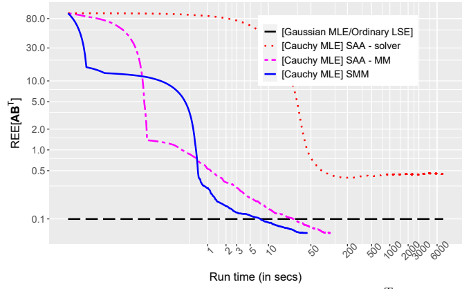
Fig. 2. Convergence comparisons for the \text{REE}[\mathbf{AB}^T] .
